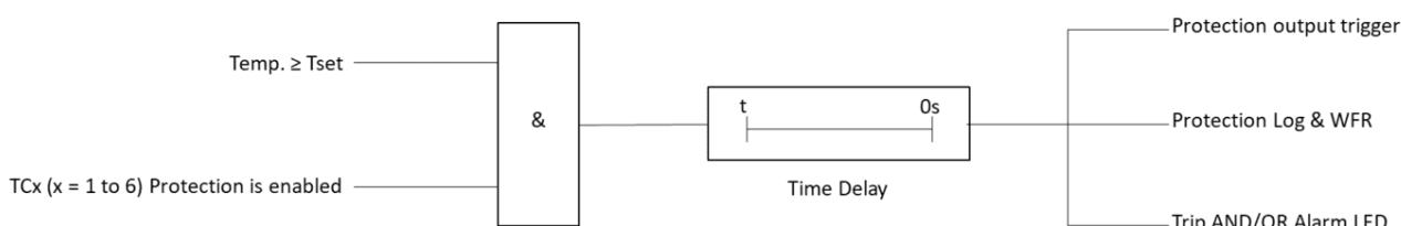
Figure 4-29 Logical Diagram of TC (Overtemperature) Protection
