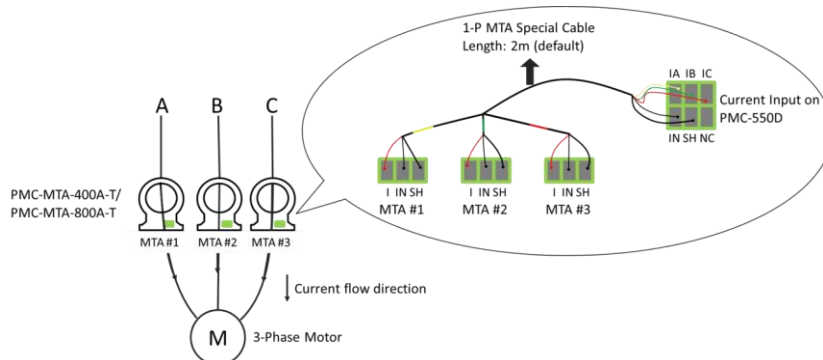
Figure 2-33 PMC-MTA-400A-T / PMC-MTA-800A-T Connections
