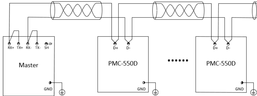
Figure 2-37 Wiring Diagram of RS-485 Communication
