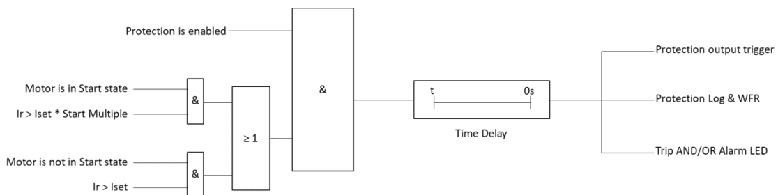
Figure 4-26 Residual Current Protection Logic Diagram
