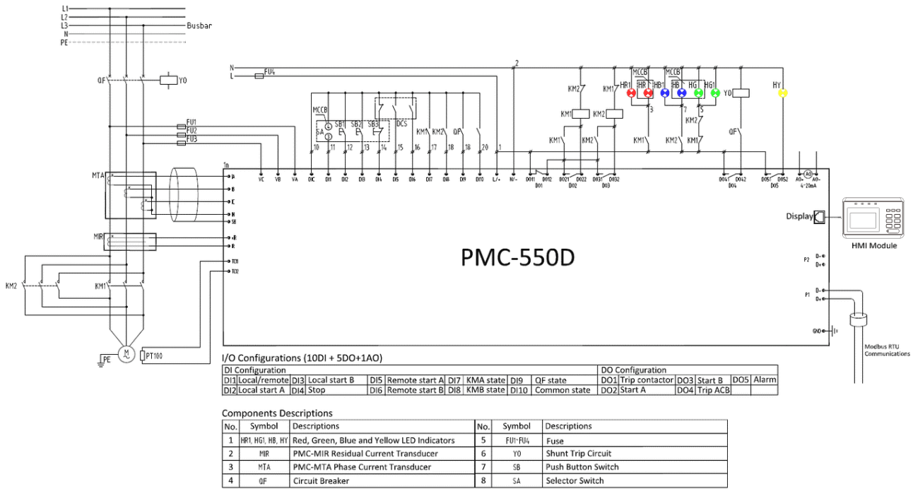
Figure 2-46 Forward / Reverse Start Operation Schematic Diagram
