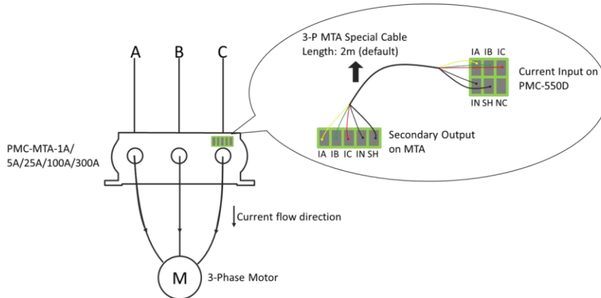
Figure 2-32 PMC-MTA-1A/5A/25A/100A/300A Connections
