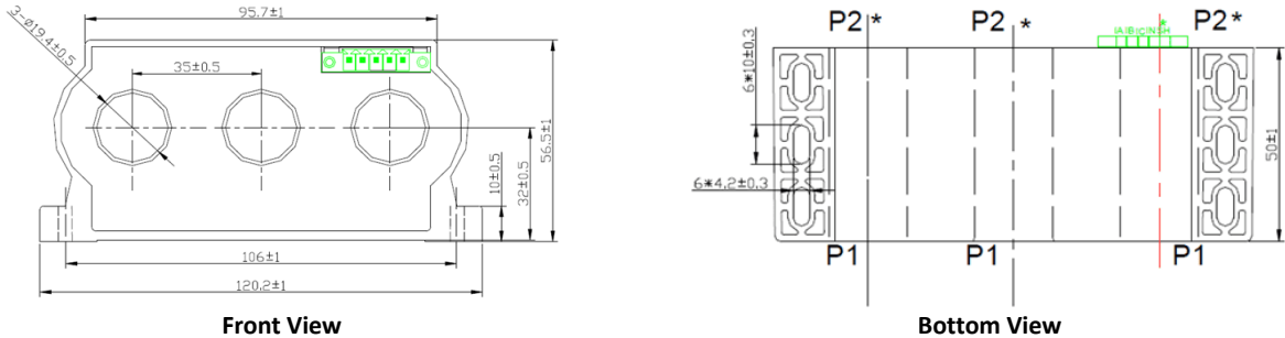
Figure 2-15 PMC-MTA-25A Dimensions
