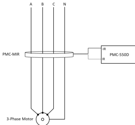
Figure 2-35 Residual Current Input Connection
