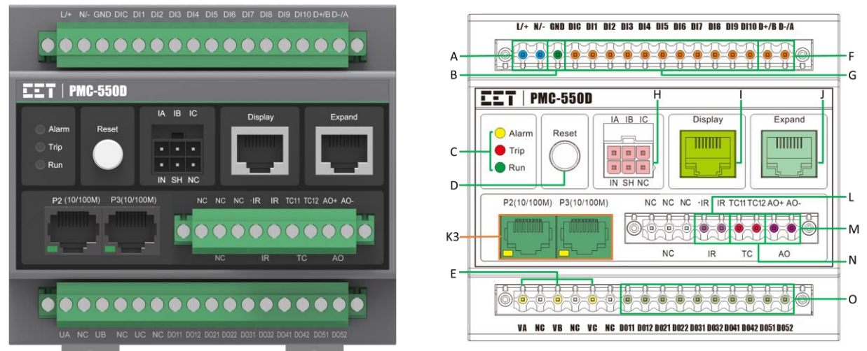
Figure 2-3 Panel View and Terminals Diagram for PMC-550D with 2x10Base-T/100Base-TX Ethernet Port
