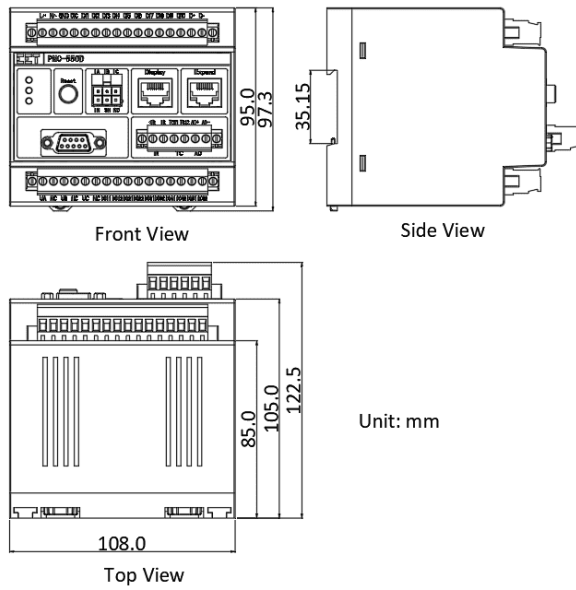
Figure 2-11 Relay's Dimensions
