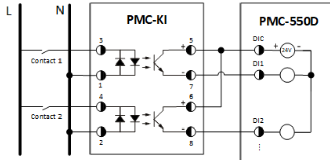
Figure 2-34 Digital Input Connection with PMC-KI Converter
