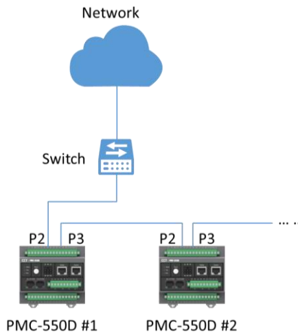
Figure 2-41 Switch Mode Connection
