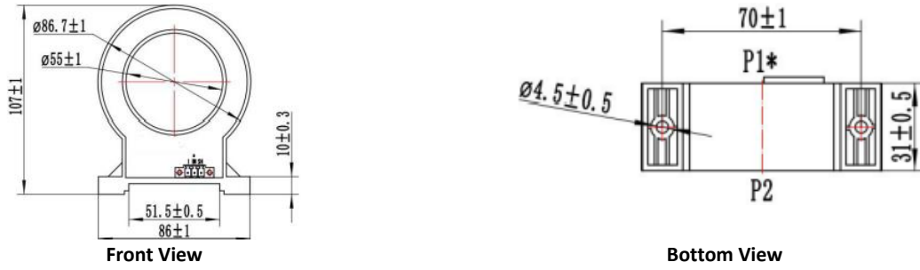
Figure 2-17 PMC-MTA-400A-T Dimensions
