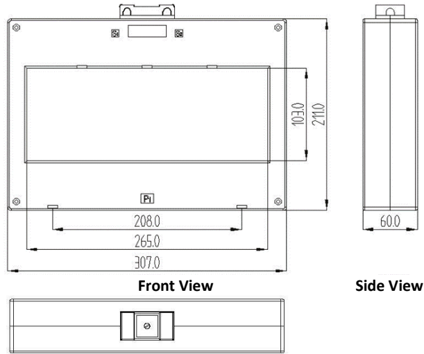
Figure 2-23 PMC-MIR-265*103 Dimensions
