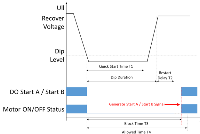
Figure 4-31 Motor Undervoltage Restart after the Undervoltage Event
