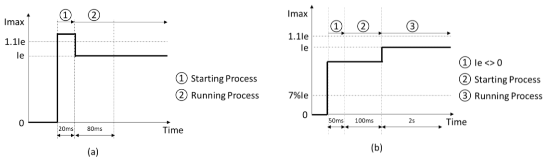
Figure 4-1 Transition between Starting and Running Processes
