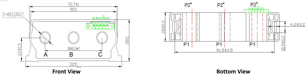
Figure 2-14 PMC-MTA-1A / PMC-MTA-5A Dimensions
