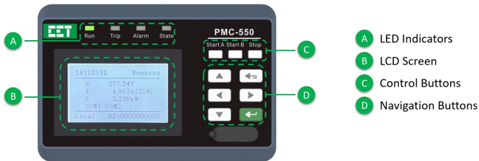
Figure 2-4 HMI Display Module
