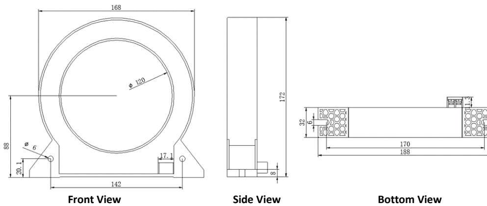
Figure 2-22 PMC-MIR-120 Dimensions
