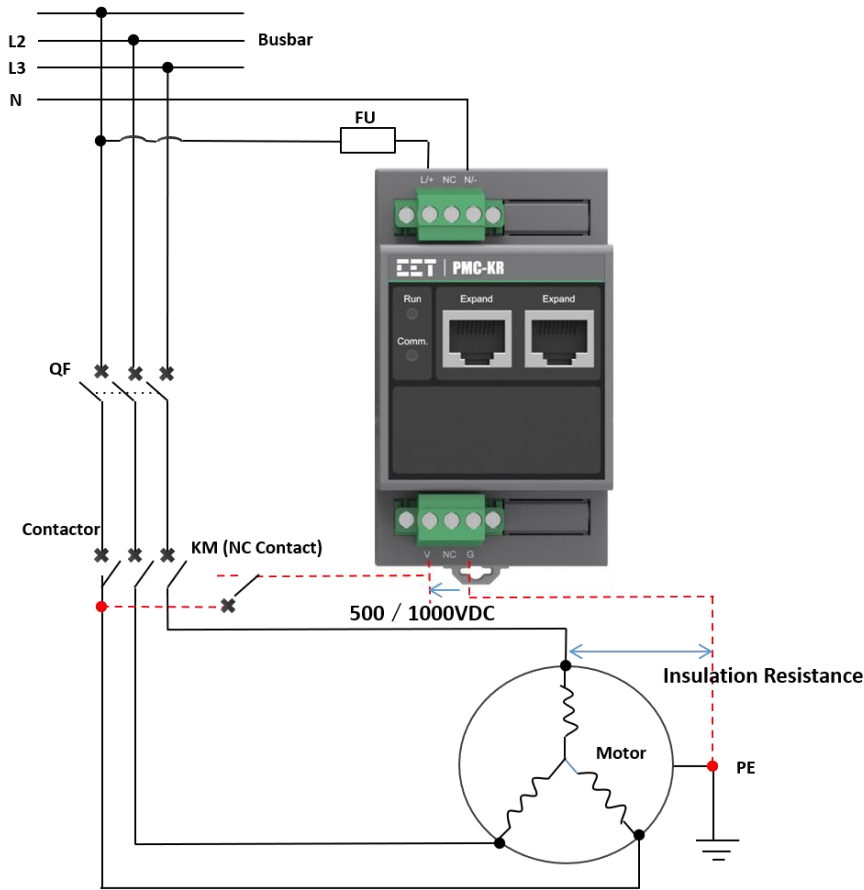
Figure 2-31 PMC-KT Connection
