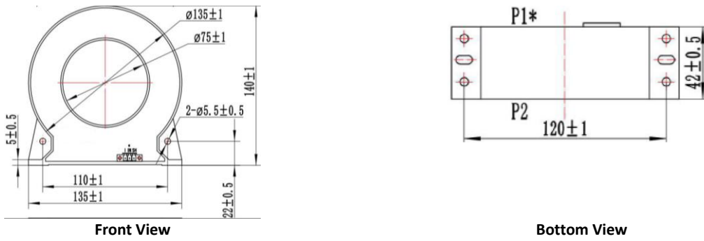
Figure 2-18 PMC-MTA-800A-T Dimensions
