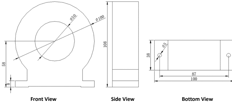
Figure 2-20 PMC-MIR-50 Dimensions
