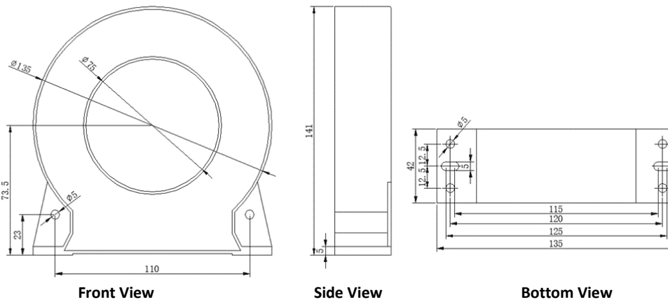
Figure 2-21 PMC-MIR-75 Dimensions
