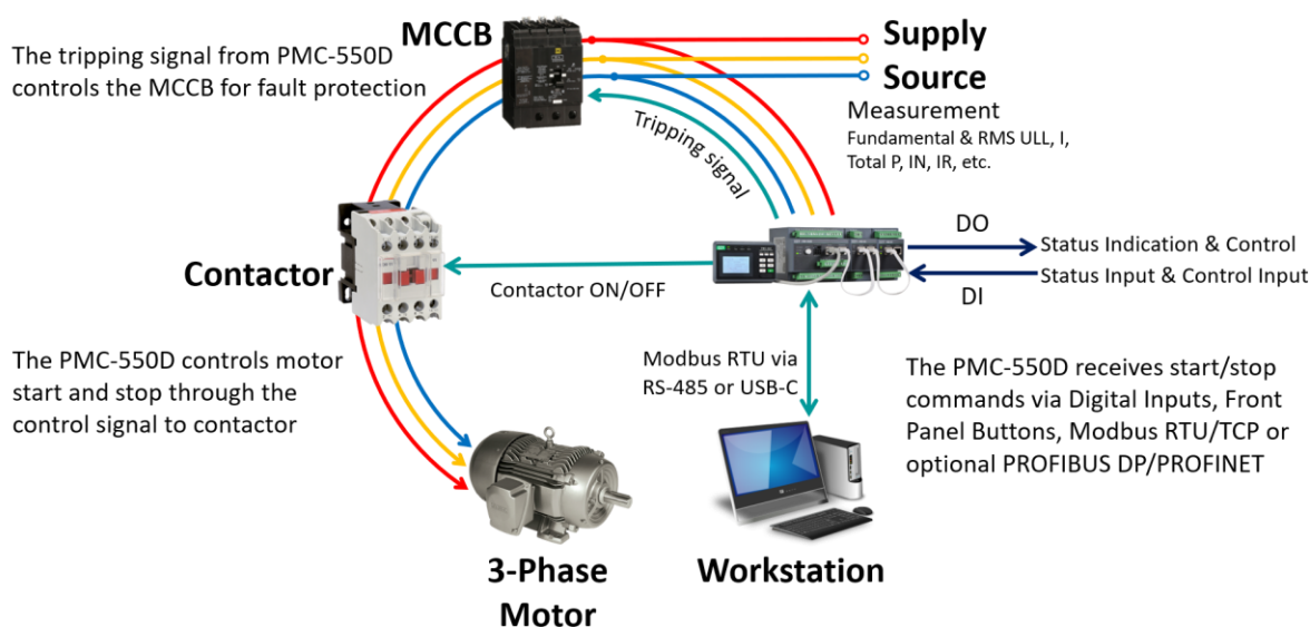
Figure 1-2 PMC-550D's Application in Motor Control and Protection Circuit
