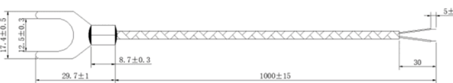
Figure 2-26 NTC-Y12 Dimensions
