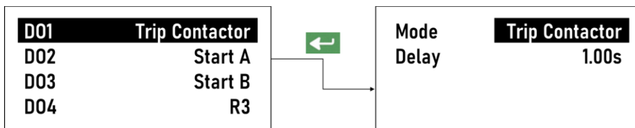
Figure 3-24 Digital Outputs Setup Screens
