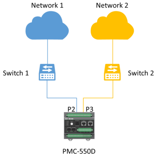
Figure 2-40 Normal Mode Connection
