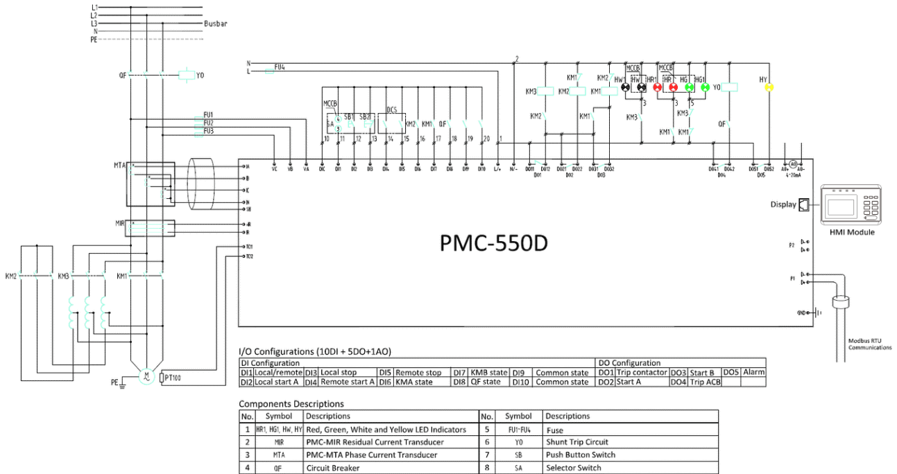
Figure 2-44 Auto-Transformer Start Operation Schematic Diagram
