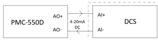
Figure 2-36 Analog Output Wiring
