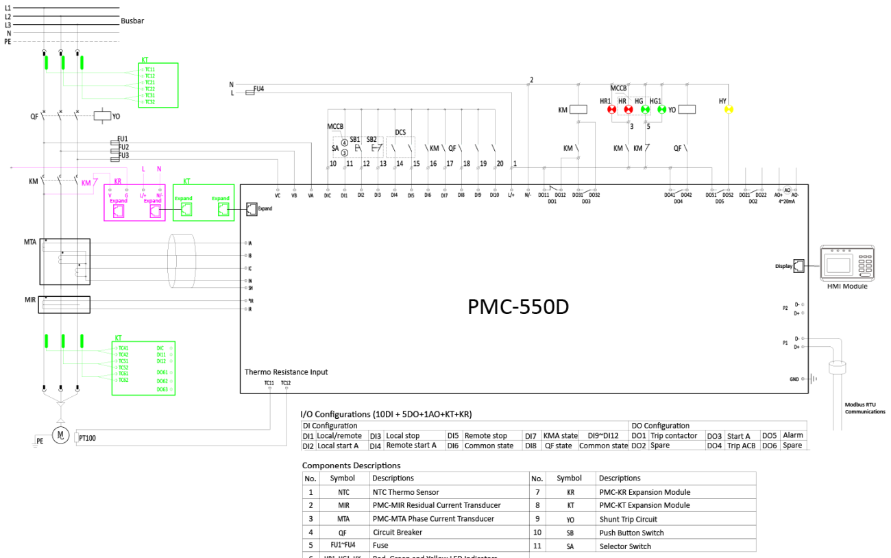
Figure 2-42 DOL Start Schematic Diagram
