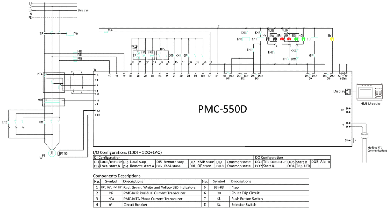
Figure 2-45 Rotor Resistance Start Operation Schematic Diagram
