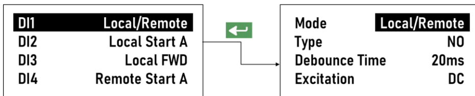
Figure 3-23 Digital Inputs Setup Screens
