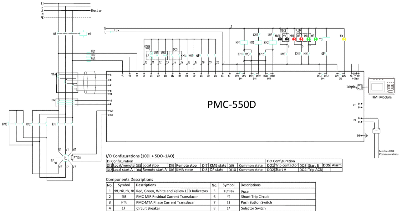
Figure 2-43 Star-Delta Start Operation Schematic Diagram
