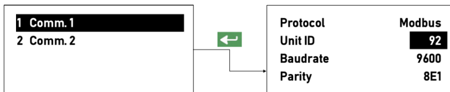
Figure 3-26 Communications Setup Screens
