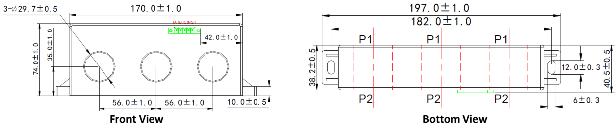
Figure 2-16 PMC-MTA-100A / PMC-MTA-300A Dimensions
