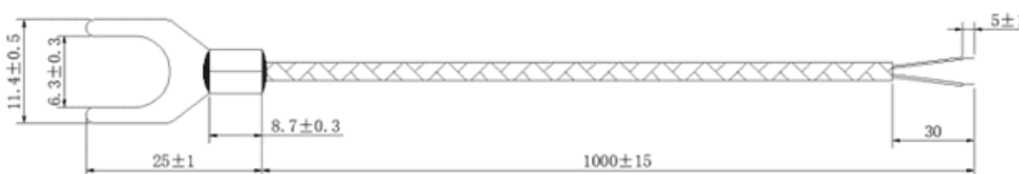
Figure 2-25 NTC-Y6 Dimensions
