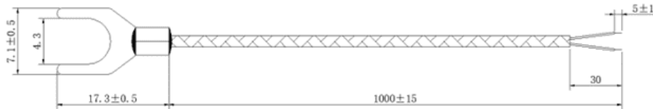
Figure 2-24 NTC-Y4 Dimensions
