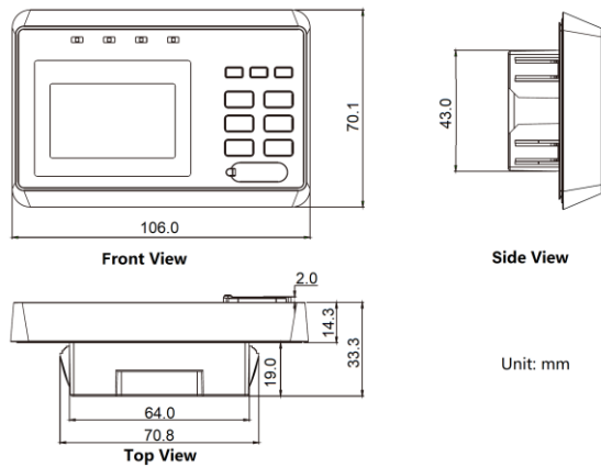
Figure 2-12 HMI Module's Dimensions
