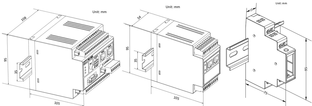
Figure 2-28 DIN Rail Mounting for Relay/Expansion Module
