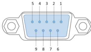
Figure 2-38 DB9 Connector Pinout
