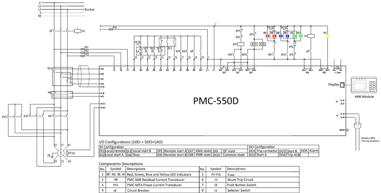
Figure 2-47 Two-Speed Start Operation Schematic Diagram
