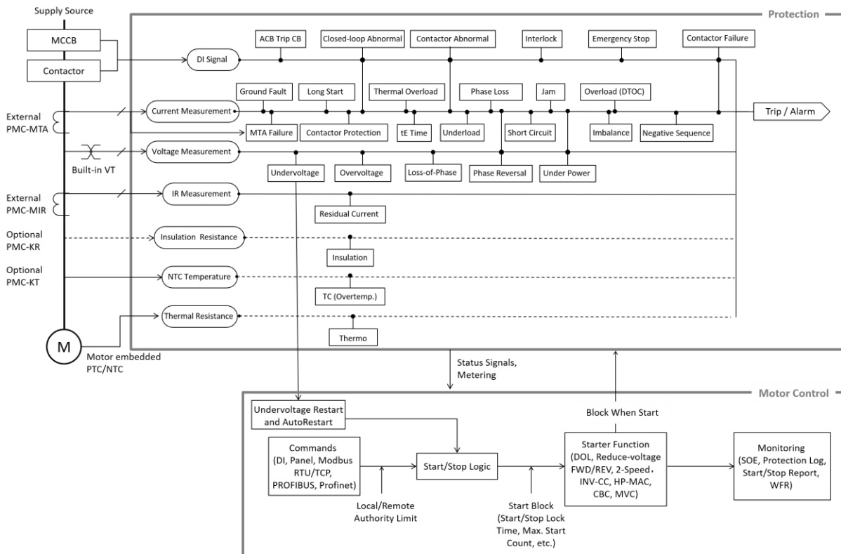
Figure 1-1 PMC-550D's Function Diagram
