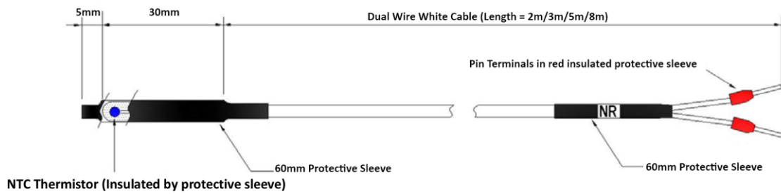
Figure 2-27 NTC-1041 Dimensions
